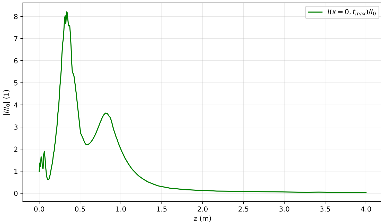
I(x=0, t_{max}, z)/I_0 , Pin=4.6Pcr
